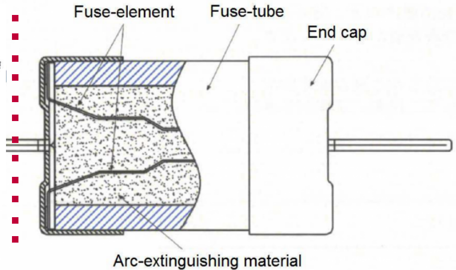
Cross section of the PT4065
